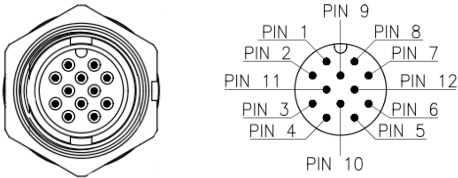
P1 PIN definition: WP-12M3-02-11 (WP B Size(M) 12PIN Front Lock )
