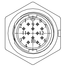
Pin Assignments Scale 2.5/1
