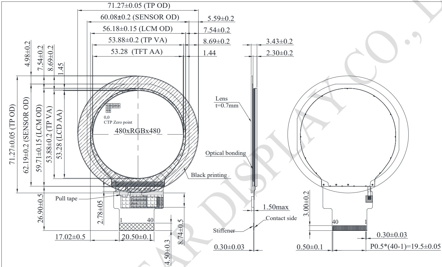
TFT FPC
