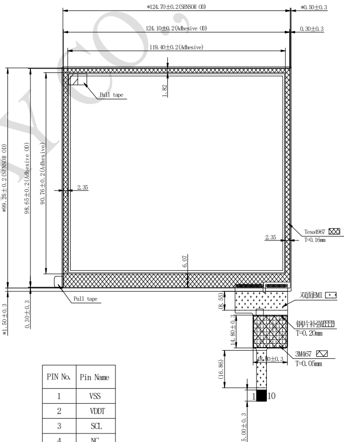
Back view
