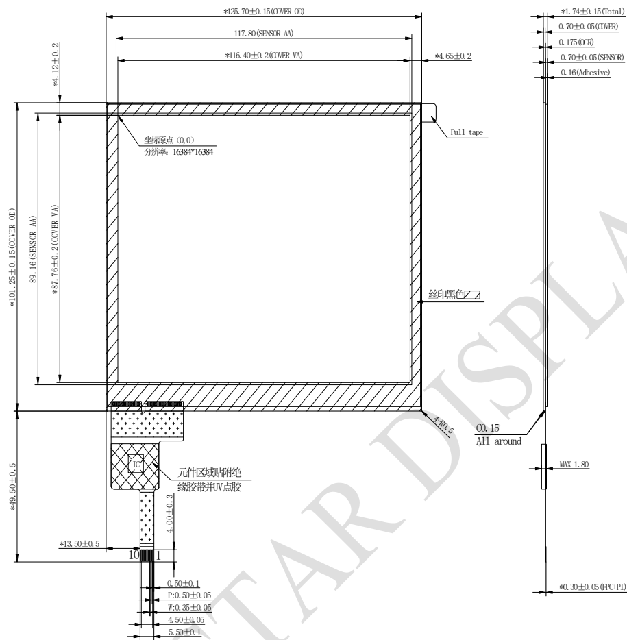
Front view
