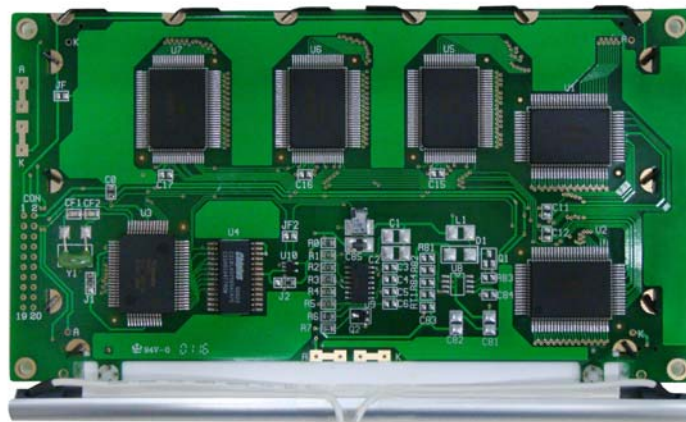
Printed Circuit Board of WG240128A
